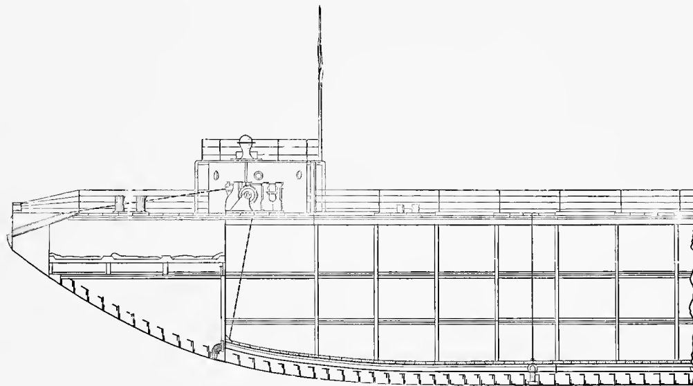
WHALEBACK STEAMER JOSEPH L. COLBY.
